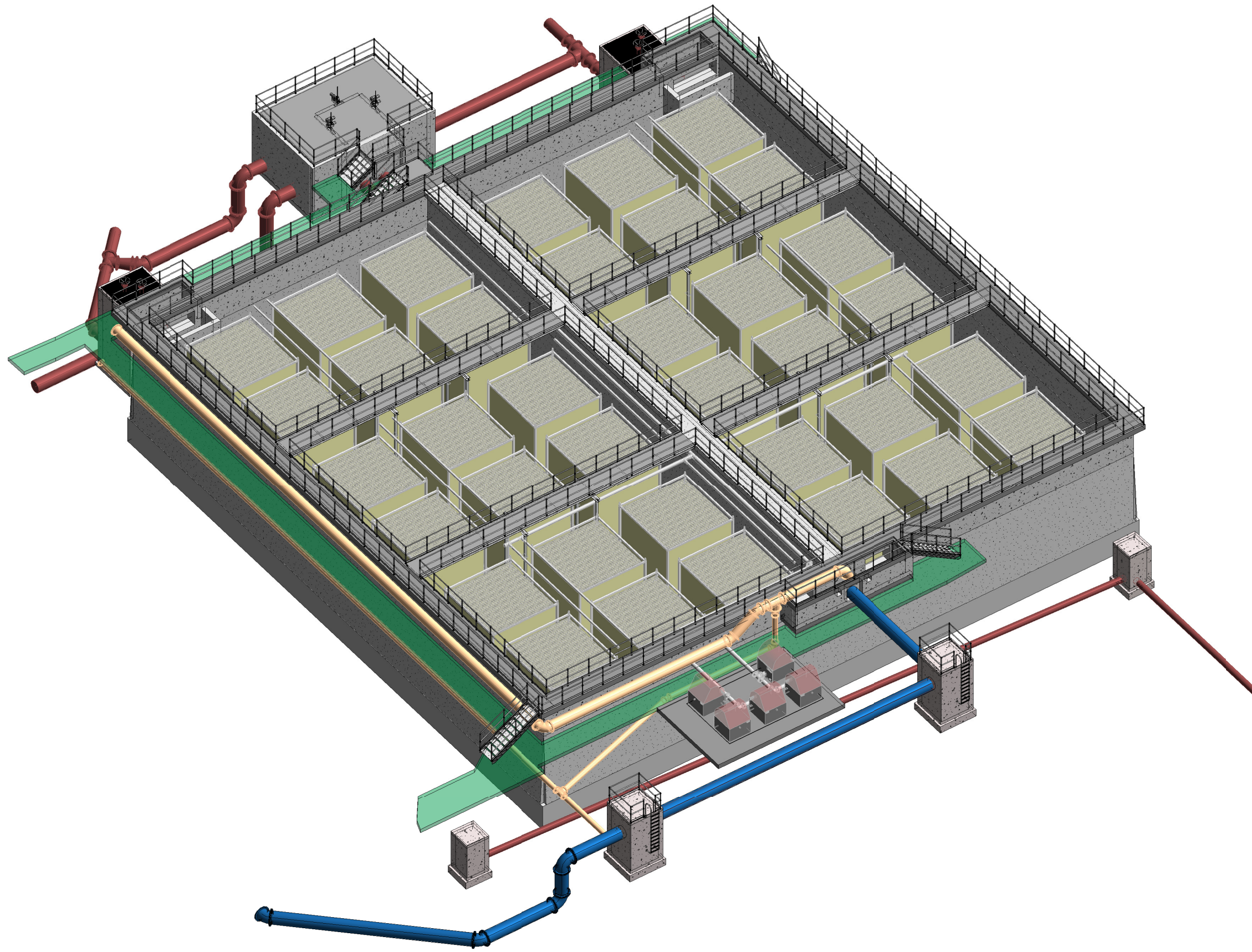
3D VIEW OF AF AERATION TANK
